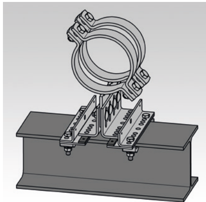
Type FG, with sliding plate
