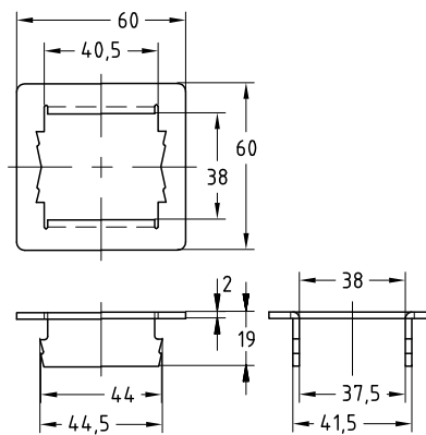
Mounting base adapter 38/40
