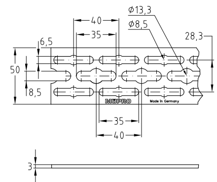
StaboFix® Section
