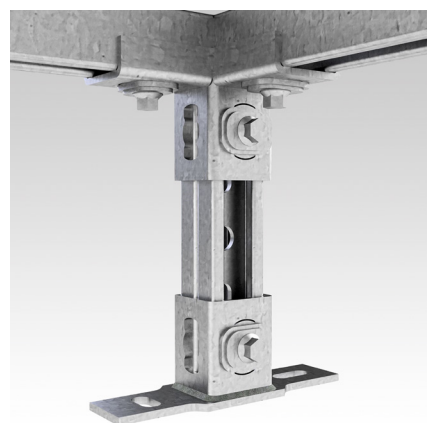
MPR-Corner connector right type S+1
