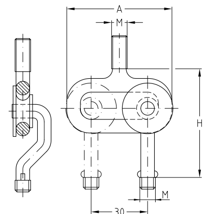
Sliding stirrup in combination with a single bossed clamp
