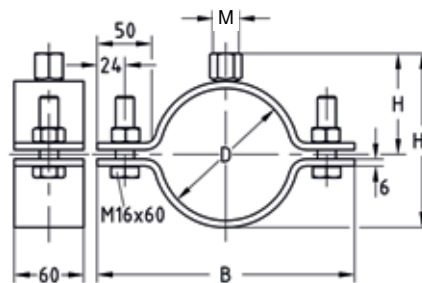
Anchor point pipe clamp 60 x 6
