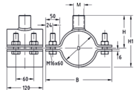
Anchor point pipe clamp 120 x 6
