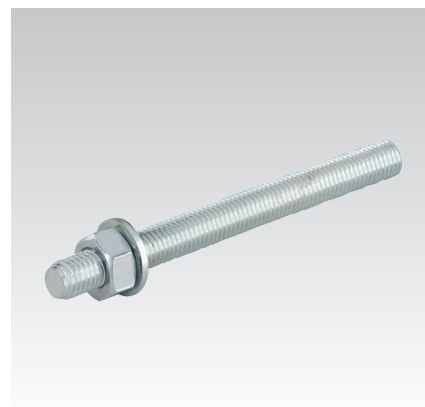
Anchor rod for solid and perforated blocks type VMU-A, strength class 5.8
