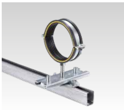
Mounting of one screw clamp with M16 cable on an MPC System rail
