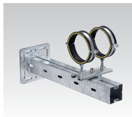
Two single bossed clamps with M16 connection threads mounted on a MPT-Console Q100
