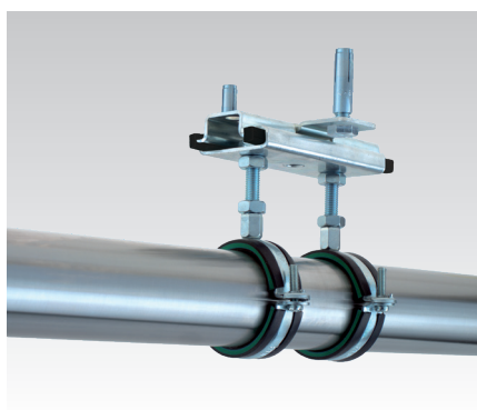
Ceiling installation with steel anchors M8
