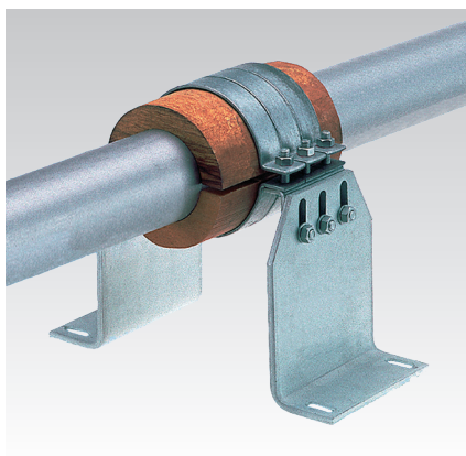
Anchor point solution on chilled water pipe with STATO® Clamps and STATO® Brackets
