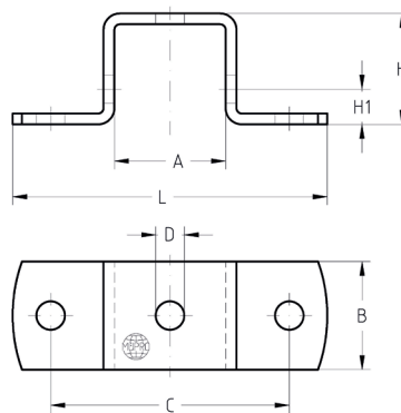
For profile 38/40
