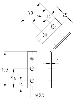
Mounting angle 45°
