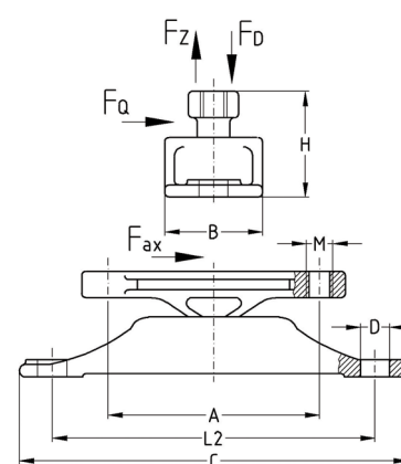
Vibration-decoupled support for equipment
