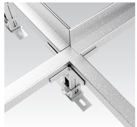
MPR-Cross connector type S+1
